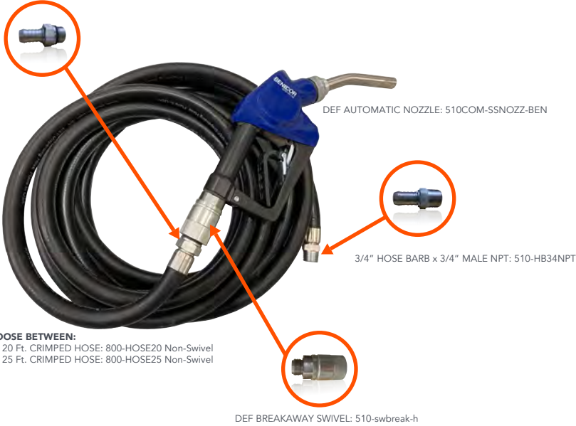
DEF BREAKAWAY SWIVEL: 510-swbreak-h
