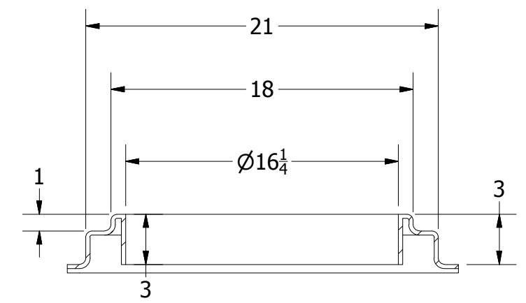
SECTION A-A SCALE 1:8
