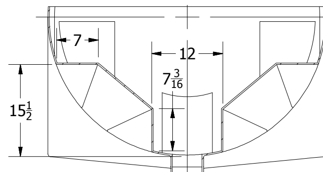
SECTION B-B SCALE 1:16
